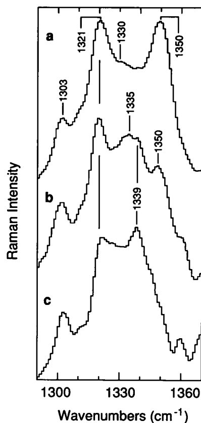
FIGURE 3 \text{C}=\text{N}-\text{H} in plane and vinylic \text{C}=\text{C}-\text{H} hydrogen bending region of (a) \text{HR}(\text{Cl}) , (b) \text{HR}(\text{NO}_3) , and (c) \text{HR}(\text{ClO}_4) blown up to magnify the differences between the two pigments. The data for \text{HR}(\text{Cl}) and \text{HR}(\text{NO}_3) are from the same set as in Fig. 1.
