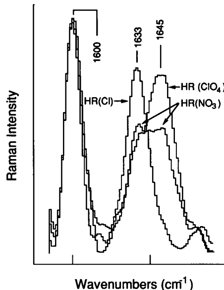
FIGURE 2 Schiff base ( \text{C}=\text{NH}^+ stretch) region of \text{HR}(\text{Cl}) , \text{HR}(\text{NO}_3) , and \text{HR}(\text{ClO}_4) blown up to show the differences between these pigments. The \text{HR}(\text{Cl}) and \text{HR}(\text{NO}_3) data are the same as in Fig 1 (spectra a and c ) except they were smoothed with a nine-point smoothing procedure. The three spectra were normalized with respect to the 1,600\text{ cm}^{-1} ethylenic bands.
